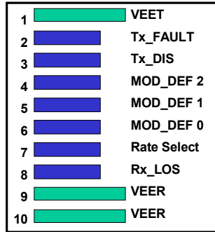
Transceiver Electrical Pad Layout Top View Bottom View
